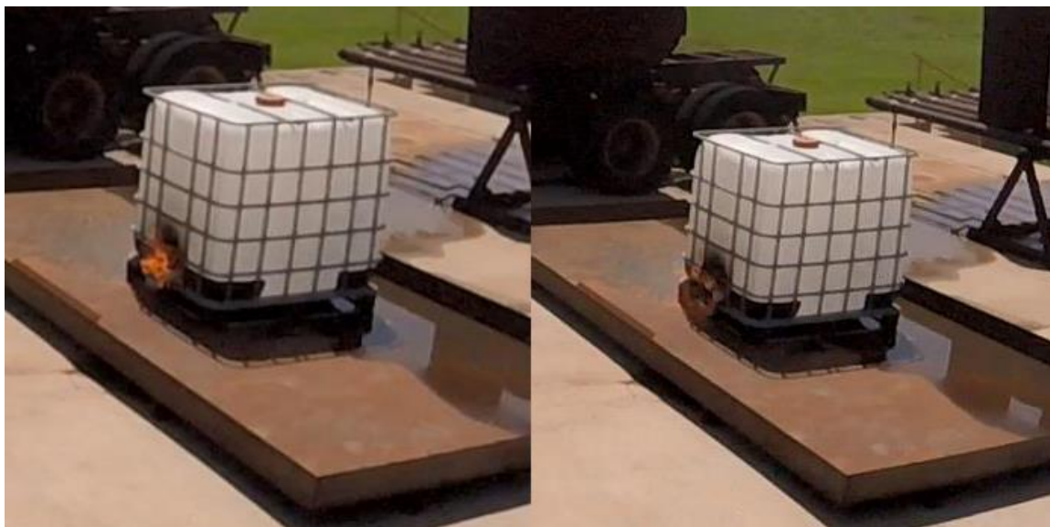
Figure 3.2: Fire from Igniter (Left) vs Fire caused by Acetone Flare-up (Right)
