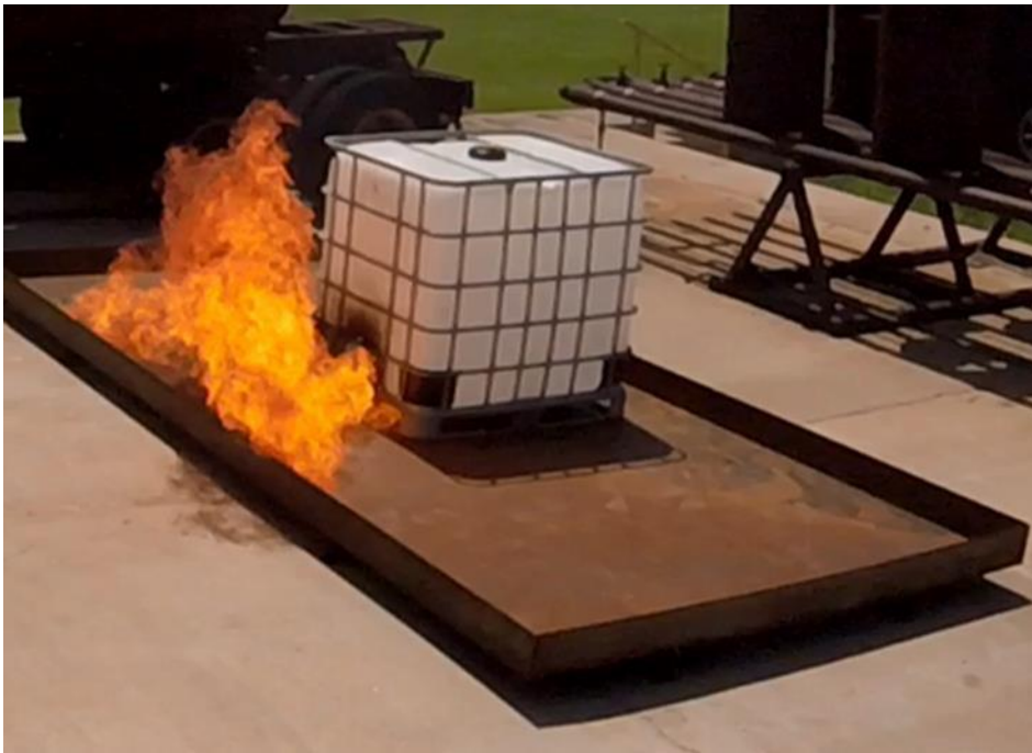
Figure 3.1: Gasoline Flare-up (2:09)
